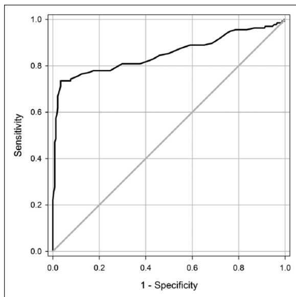
Figure 6. Receiver operating characteristic (ROC) curve for automated ABI device in diagnosing PAD as defined by ultrasound duplex scan. Area under curve=0.88 (95% CI: 0.83–0.93, p<0.001 ). ABI: ankle brachial index; CI: confidence interval; PAD: peripheral arterial disease.
